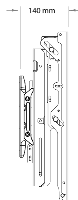
The distance with P-Bar + P-Wall Bracket
